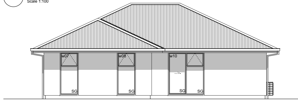
E-03 East Elevation Scale 1:100
