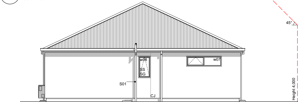
E-03 South Elevation Scale 1:100
