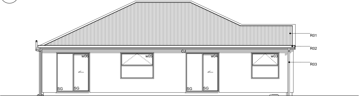
E-02 West Elevation Scale 1:100
