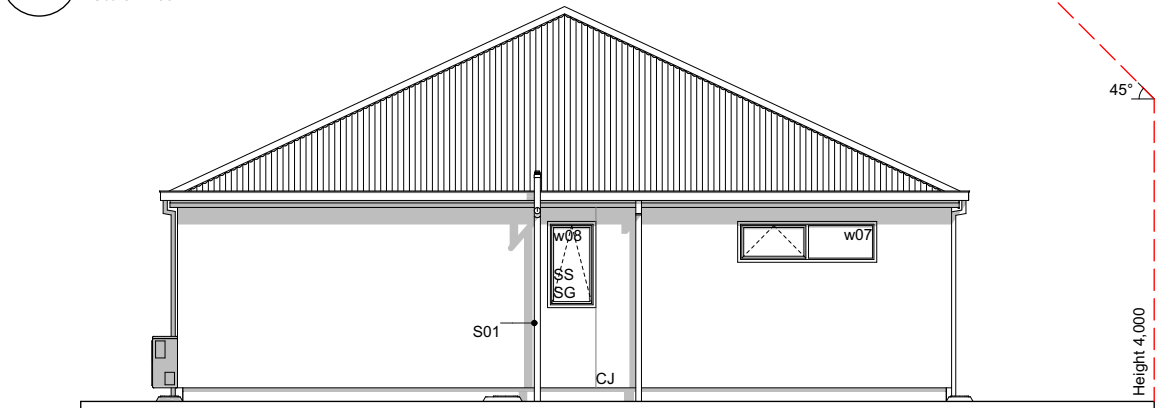
E-03 South Elevation Scale 1:100
