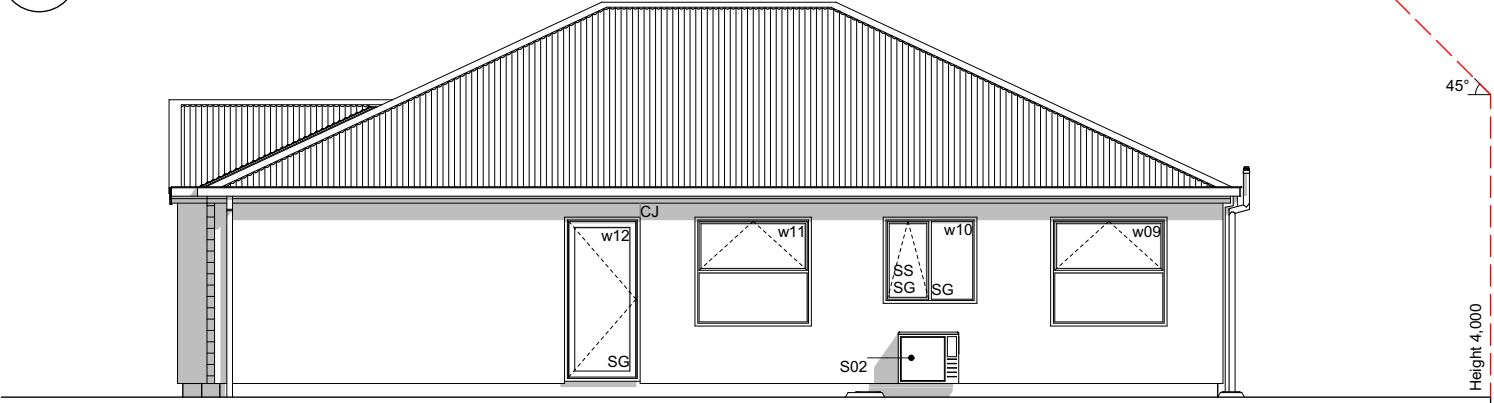
E-04 East Elevation Scale 1:100
