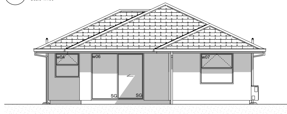
E-03 North Elevation Scale 1:100
