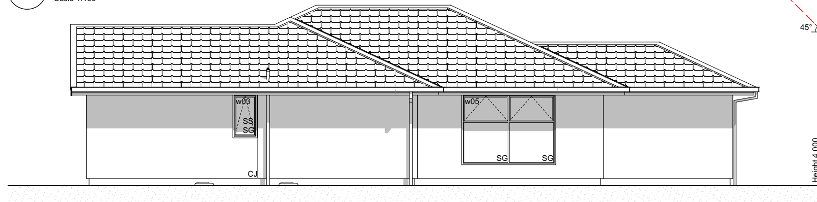
E-02 East Elevation Scale 1:100
