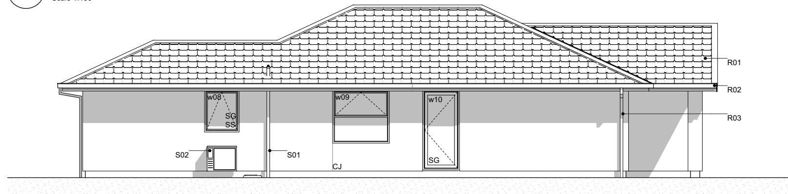
E-04 West Elevation Scale 1:100
