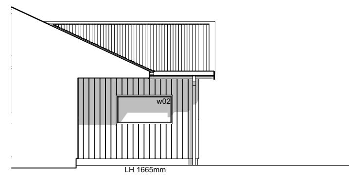
E-05 East Elevation 2 Scale 1:100
