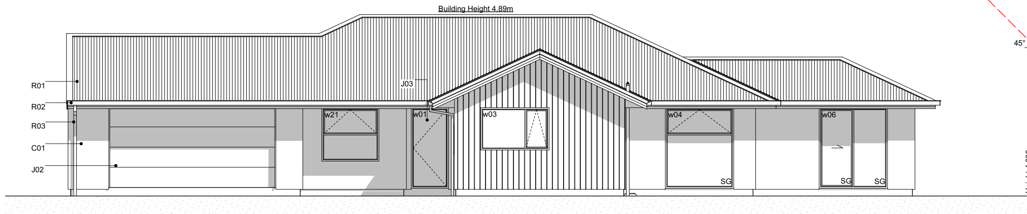
E-01 North Elevation Scale 1:100
