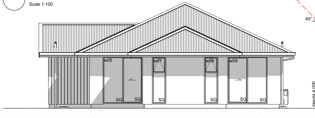
E-02 West Elevation Scale 1:100
